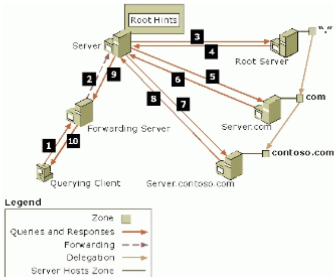
Figure 19: Forwarding example.
