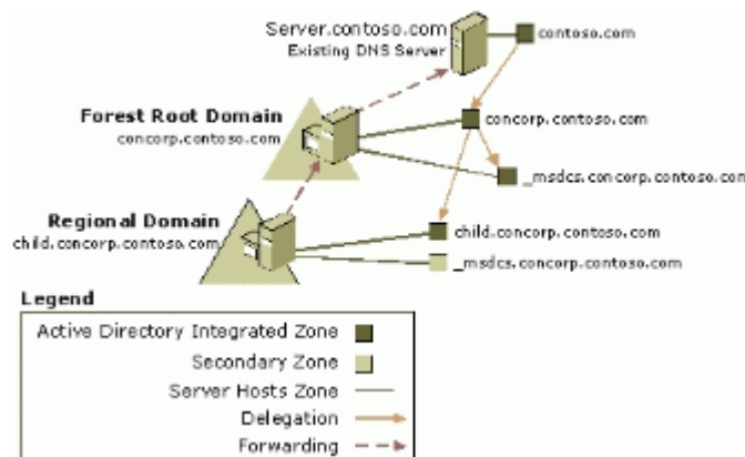
Figure 24: Integration with existing service using forwarding
