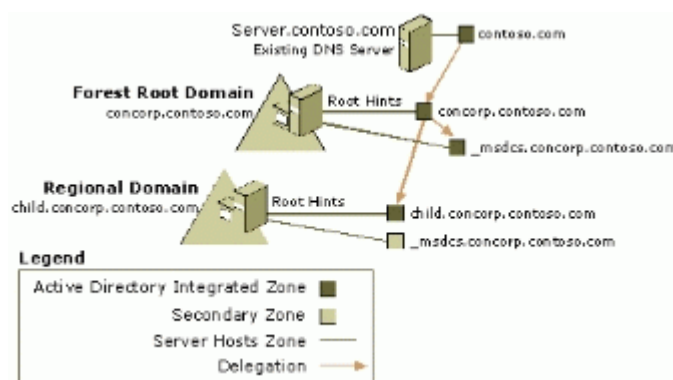
Figure 23: Integration with existing service using root hints
