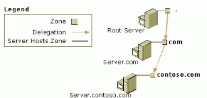
Figure 17: Delegation example.
